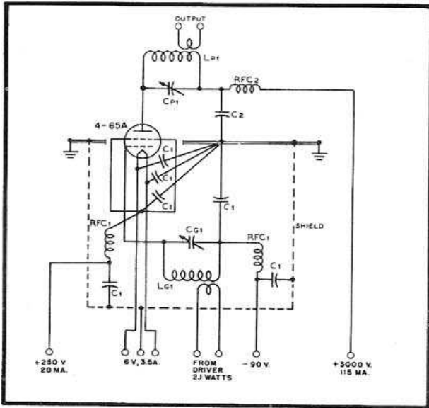
Typical radio-frequency power amplifier circuit, Class-C telegraphy, 345 watts input.
