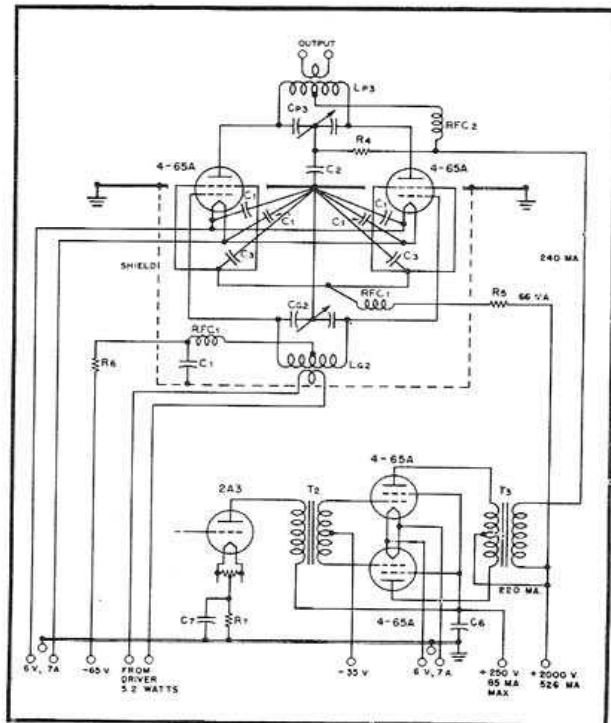
Typical high-level-modulated R-F amplifier circuit, with modulator and driver stages, 480 watts plate input.
