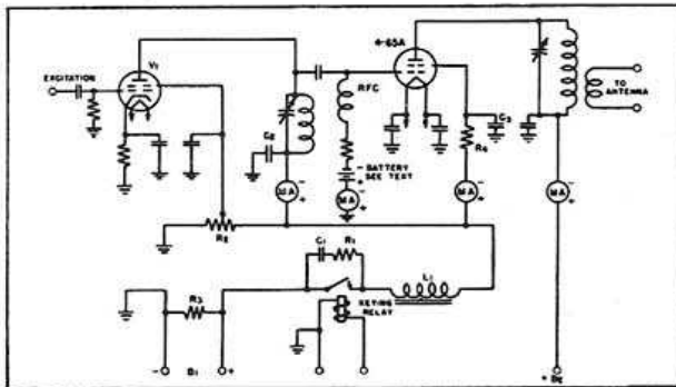
Tetrode Keying Circuit
